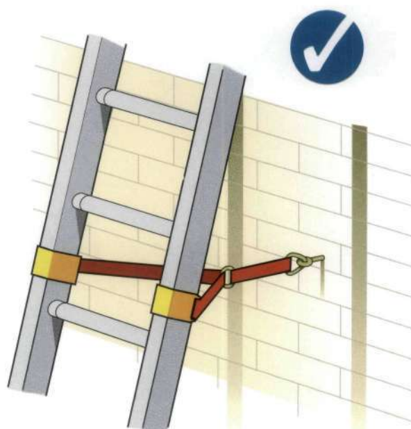
Figure 18c Tying at base
