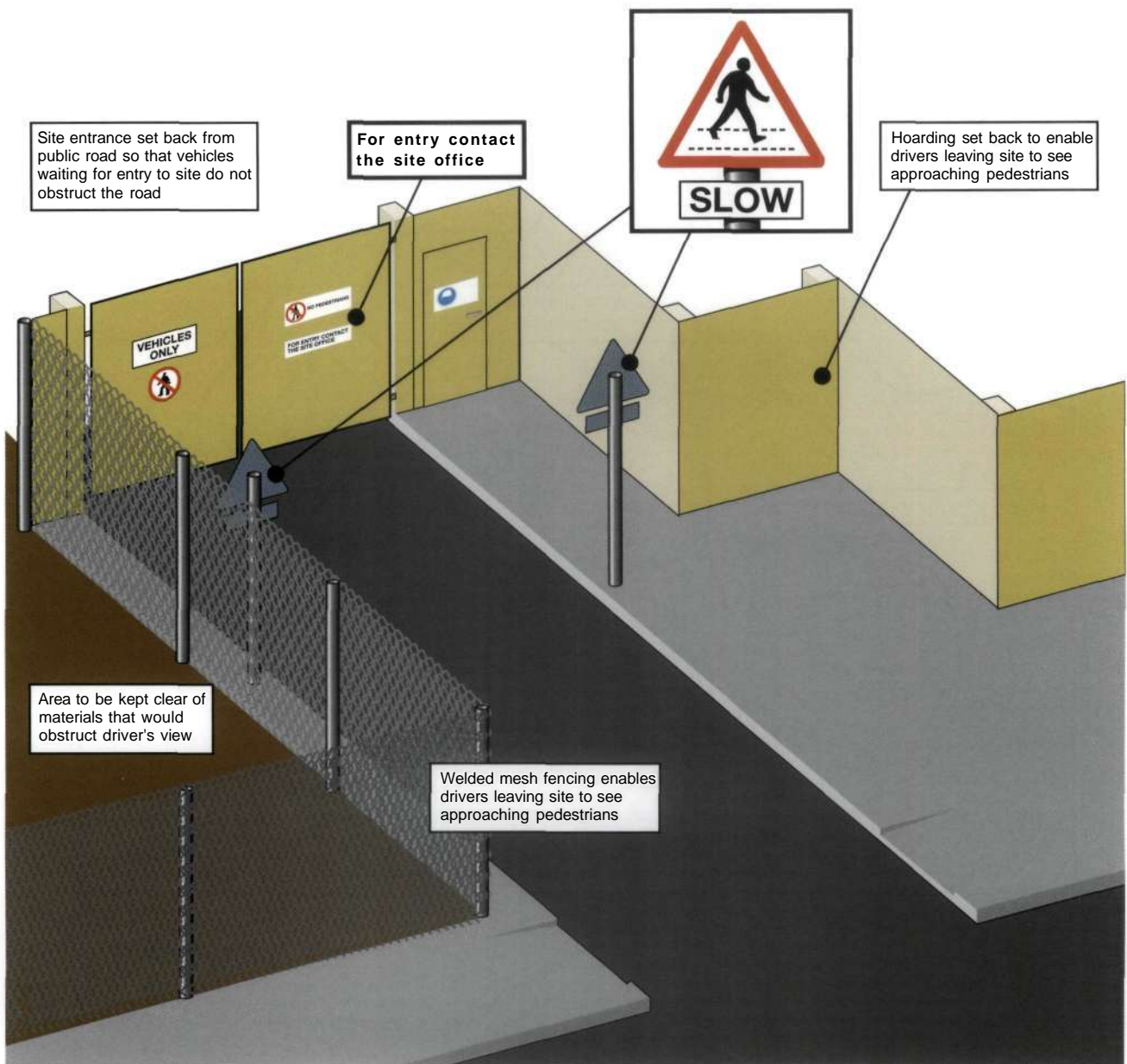
Figure 31 Use gates or barriers etc to control entry into the work area and display the procedure for obtaining entry
