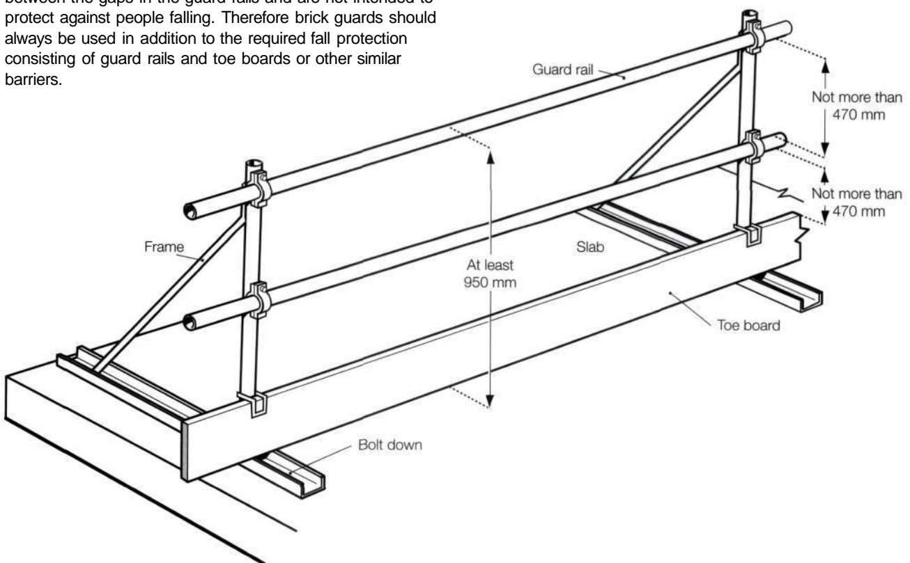
Figure 10 Guard rails and toe boards
