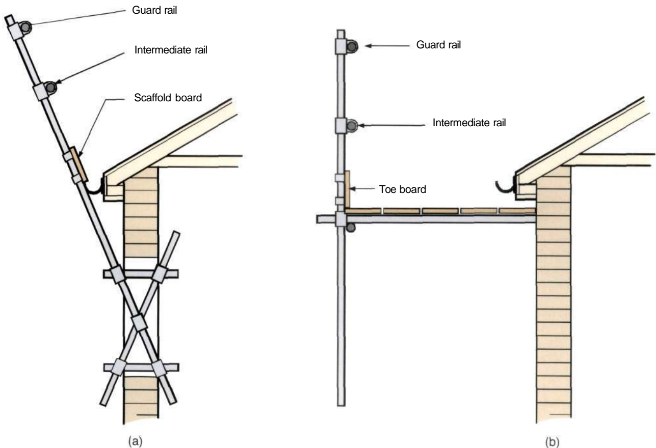
Figure 23 Typical sloping-roof edge protection
