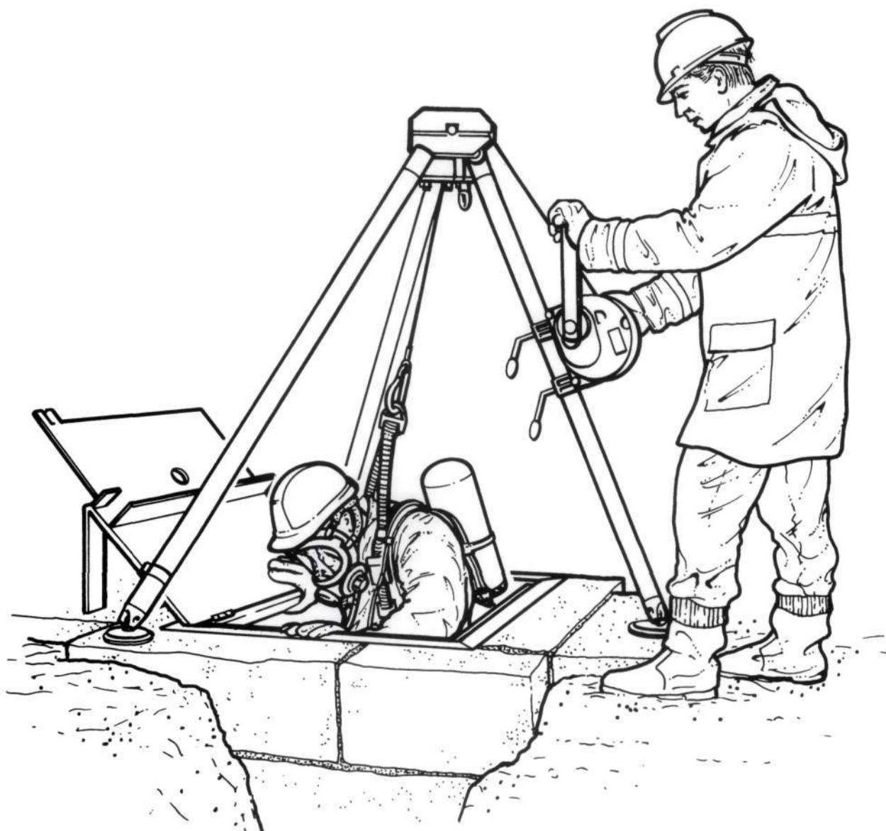
Figure 51 A worker wearing full breathing apparatus is also wearing a harness and lanyard connected to a winch so that he can be hauled to the surface in an emergency without others having to enter the manhole to rescue him
