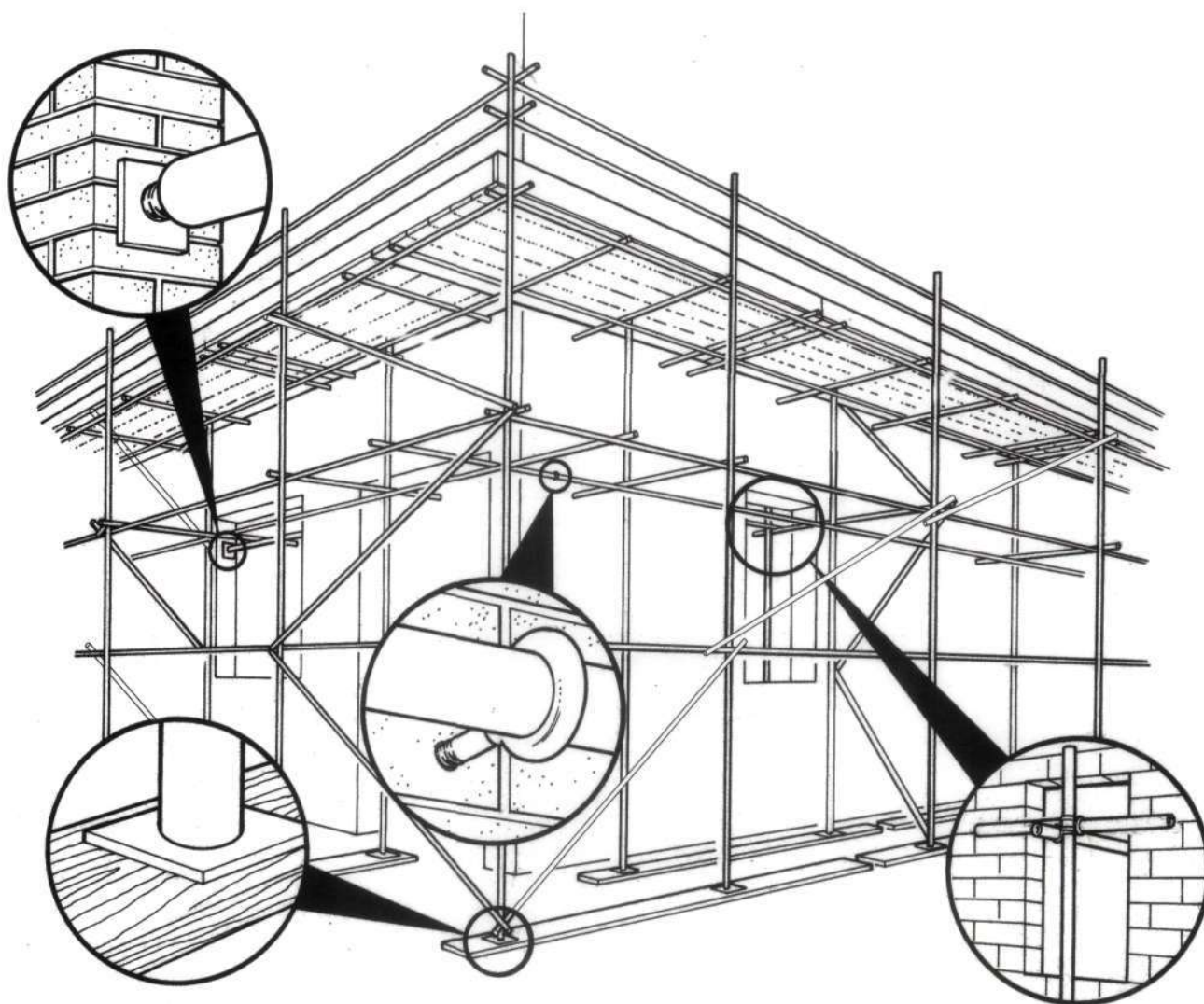
Figure 9 An independent scaffold
