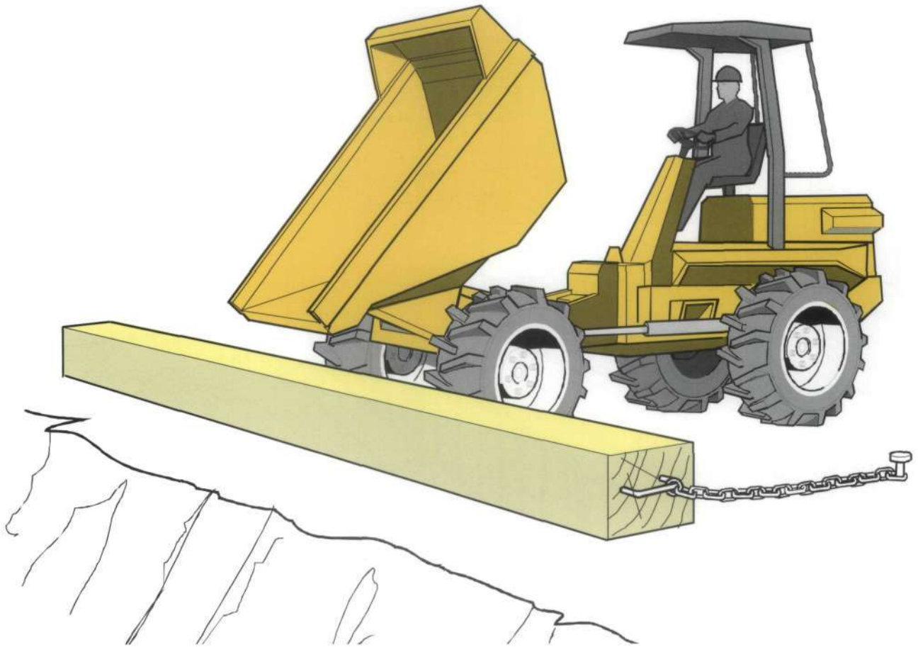
Figure 35 Take precautions, such as stop blocks, where vehicles tip materials into excavations
