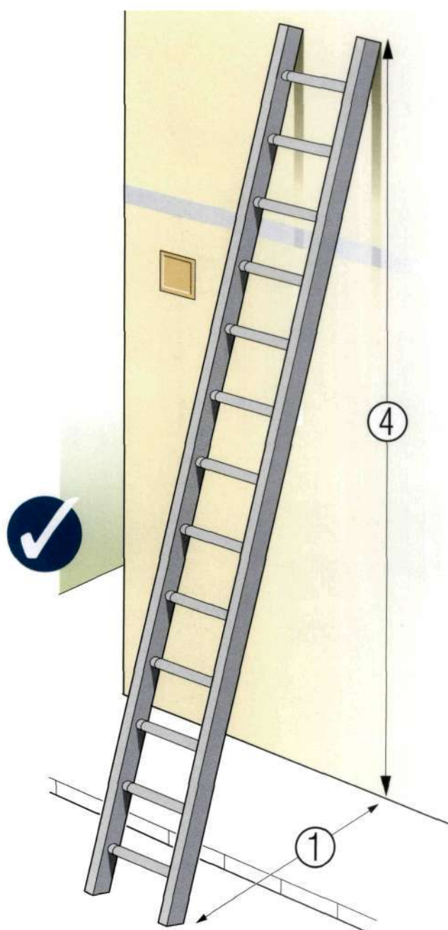
Figure 19 Ladder showing correct 1 in 4 angle (means of securing omitted for clarity)
