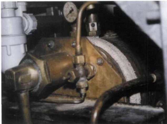
Figure 48f Asbestos rope seal in a domestic gas boiler
