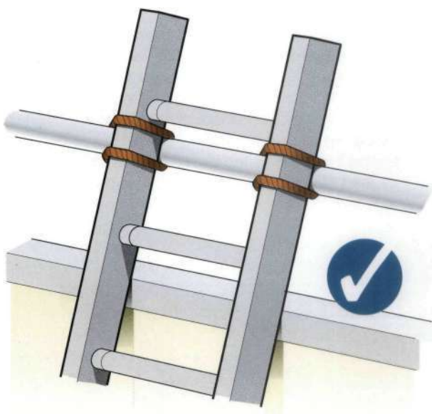
Figure 18a Ladder tied at top stiles (correct for working on, not for access)
