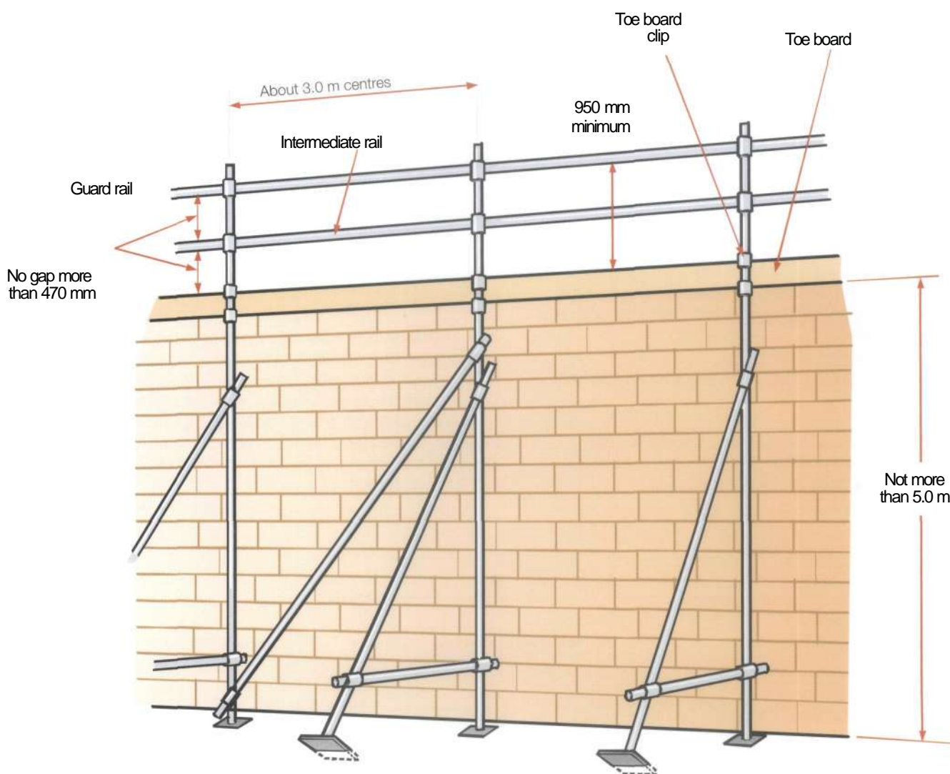
Figure 24 Example of flat-roof edge protection
